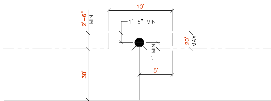
FIRE HYDRANT EASEMENT DETAIL
